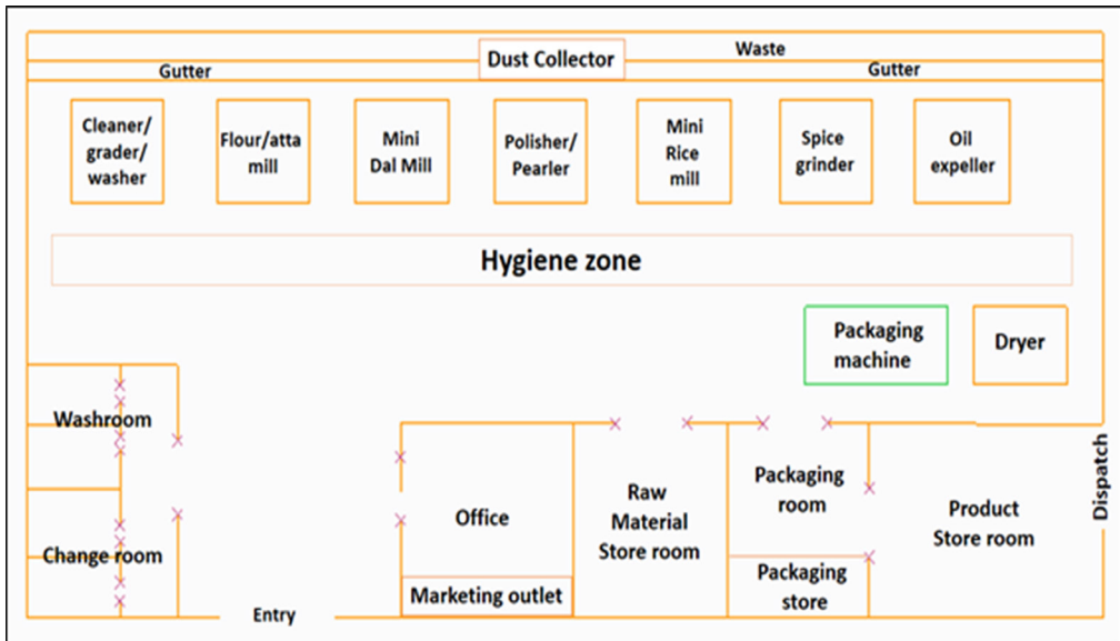
Fig. 1. A typical layout of agro-processing centre
